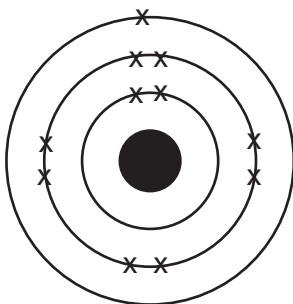
sodium atom as 2, 8, 1 [1]
