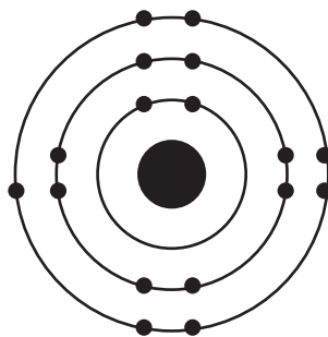
chlorine atom as 2, 8, 7 [1]
